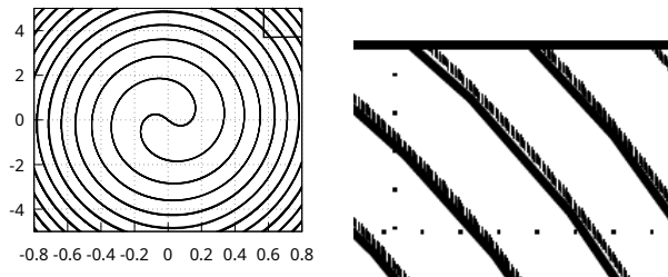
Figure: Here one can see the cross-section of the u, u' bifurcation boundary at x = -50 for solutions of the non-linearly perturbed Painlevé-2 equation (9) at \varepsilon = 0.1 . The boundary obtained numerically for 2048 \times 4096 trajectories, with the beginning at x = -50 , and the boundary calculated from perturbation theory almost coincide. Differences can be observed away from the center. The rectangle highlighted in the left drawing is enlarged in the right drawing. In the right drawing, the boundary obtained numerically corresponds to short vertical dashes, the boundary obtained by perturbation theory is indicated by continuous lines.
